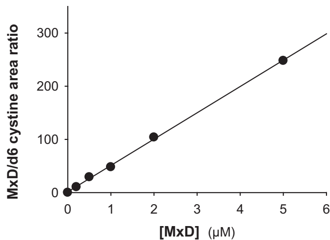
Fig. 56. Calibration curve of the mixed disulfide (MxD) liquid chromatography tandem MS assay. Increasing dilutions from a known MxD solution were tested. The assay is linear up to 5 μM ( R^2 = 0.9992 ).
